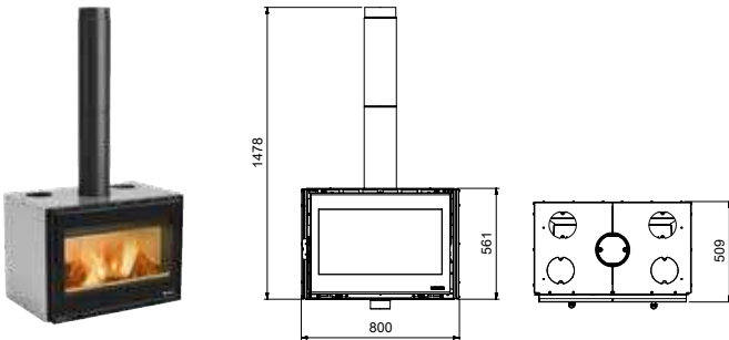
Technical Drawing
