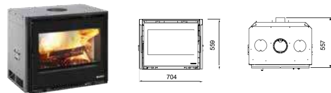
Technical Drawing
