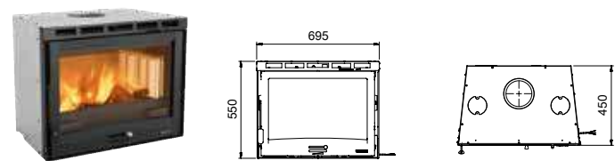
Technical Drawing
